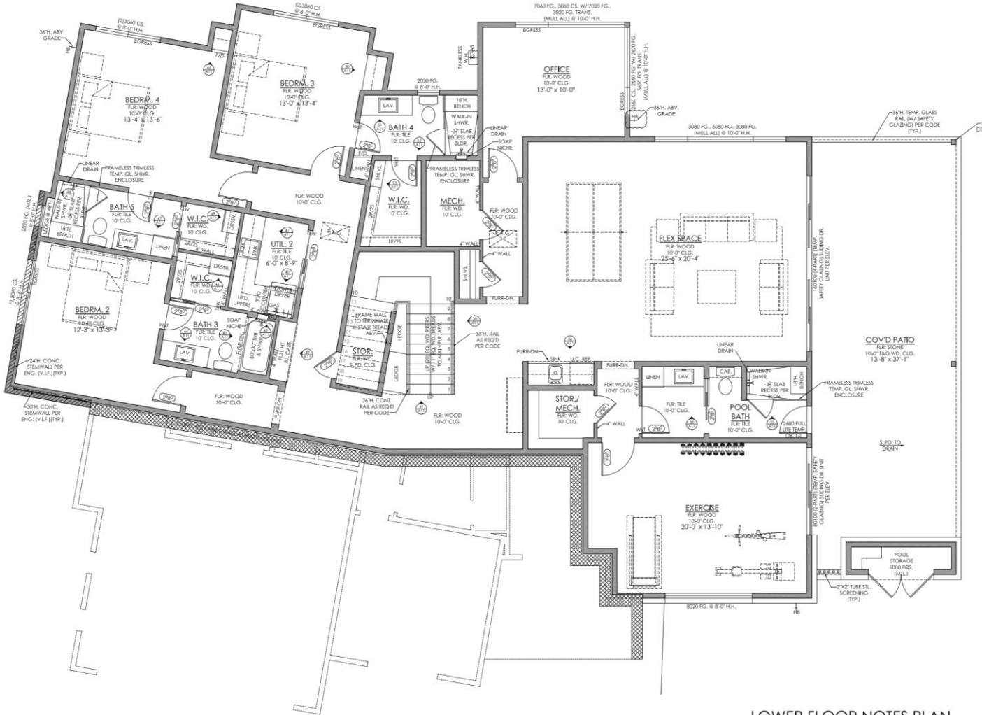
LOWER FLOOR NOTES PLAN
